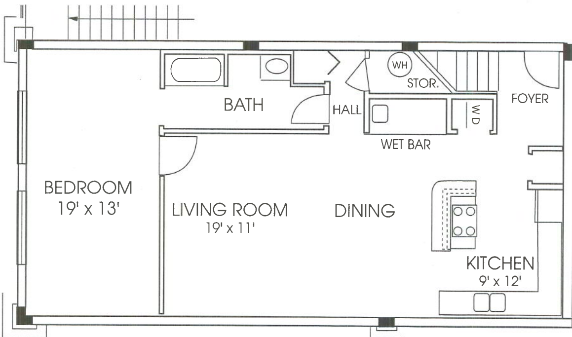
FIRST LEVEL FLOOR PLAN
