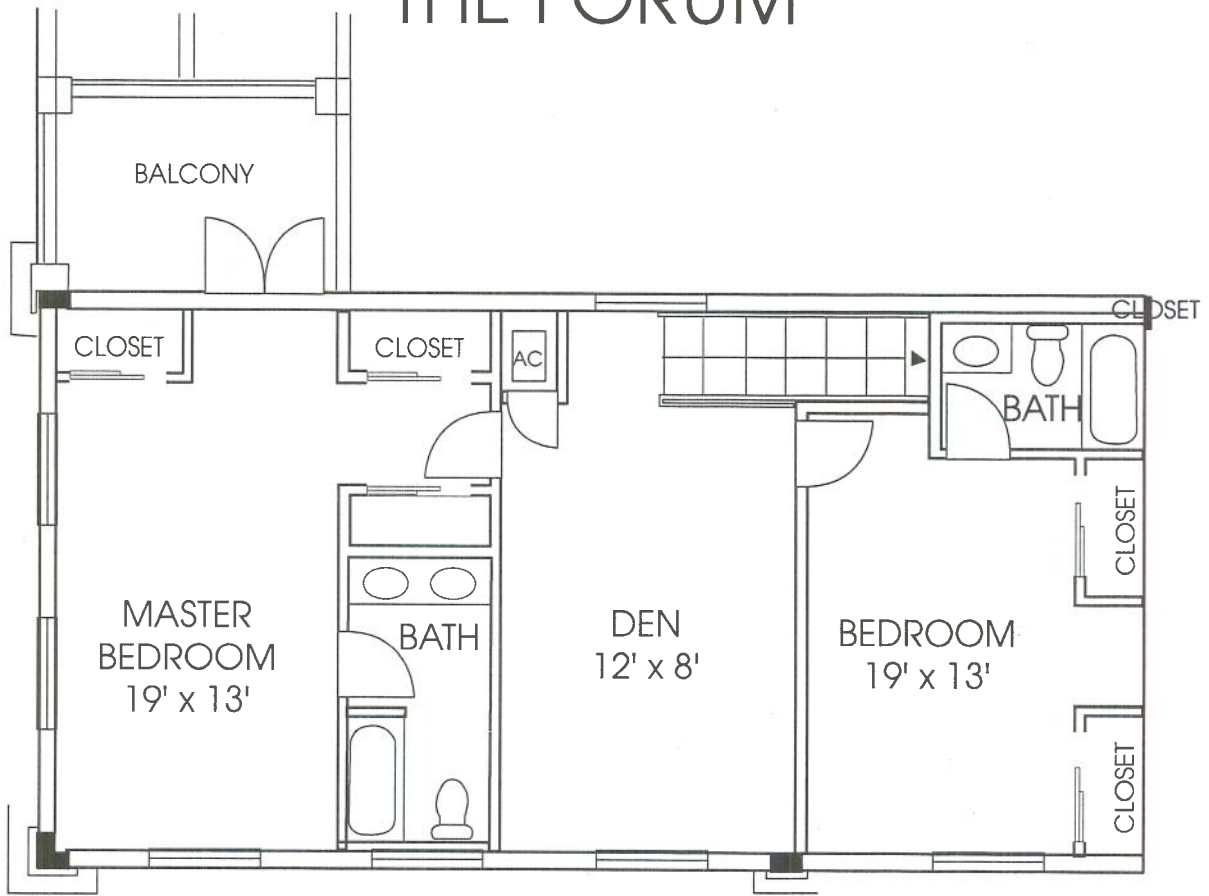
SECOND LEVEL FLOOR PLAN
