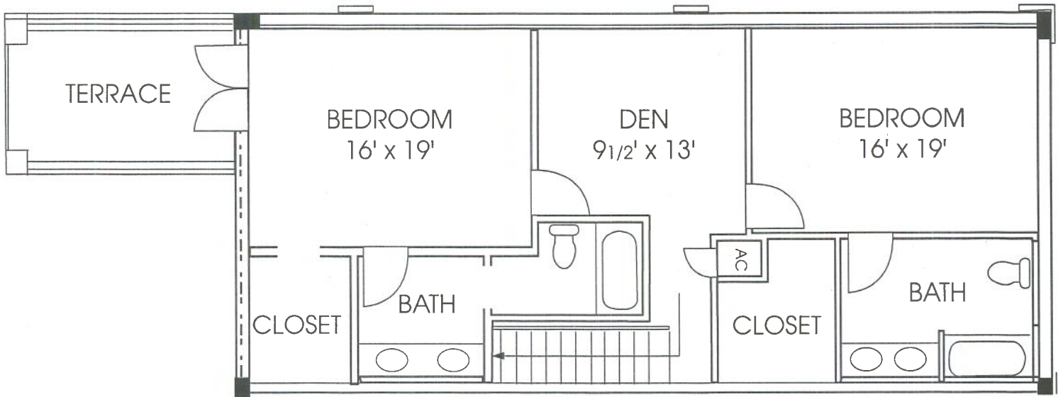
SECOND LEVEL FLOOR PLAN
